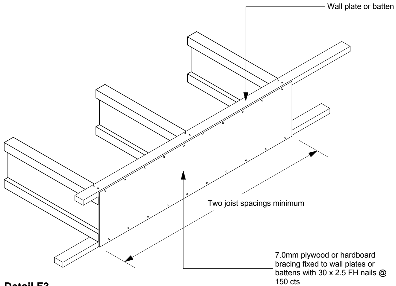
Detail F3 End restraint - using ply or hardboard bracing Scale: NTS May 2007
