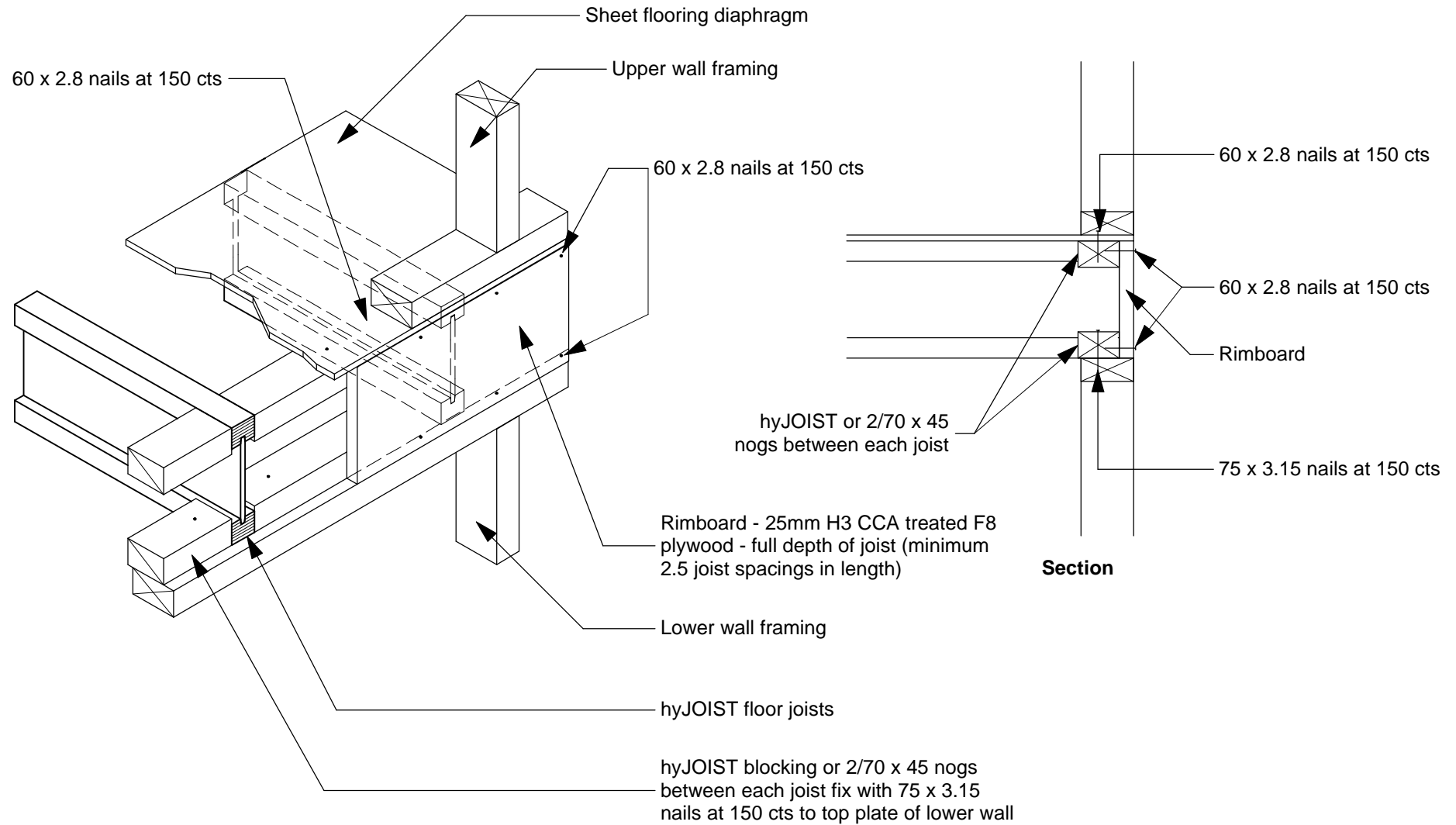
Detail TD5 Bracing transfer through diaphragm floors Scale: NTS May 2007
