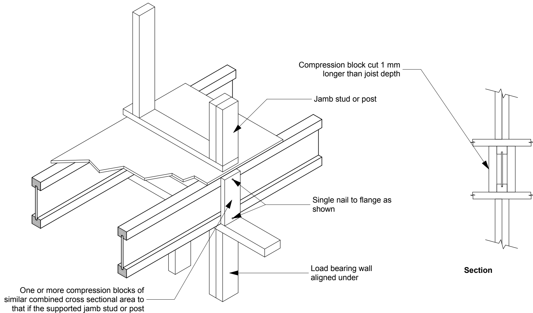
Detail F18 Installation of compression blocks Scale: NTS May 2007
