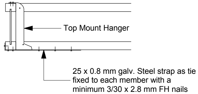
Detail F10 hyJOIST / hyJOIST connection May 2007
